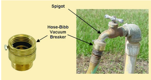
Figure 1: Hose Bibb Vacuum Breaker Example
